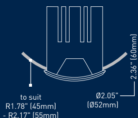
LEDpod XL50 R50
