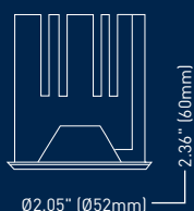
LEDpod XL50 Flat
