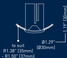
LEDpod XL28 R35
