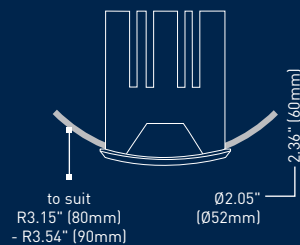
LEDpod XL50 R85
